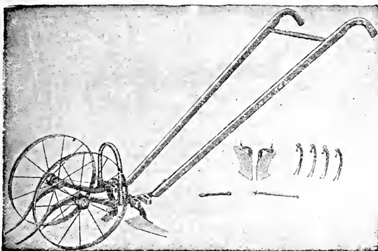
No. 301 "Iron Age" Double and Single Wheel Hoe
